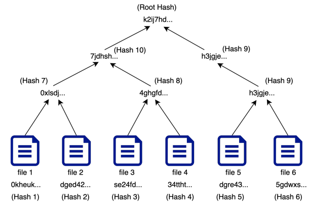
Figure 3: Example of a Merkle Hashing
